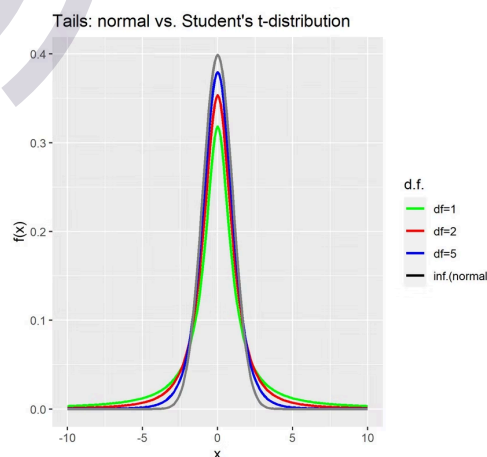
Figure 3: Normal vs. Student's t-distribution Tails
